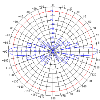
E Plane
