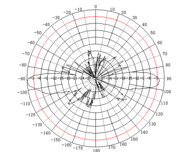
5GHz E Plane
