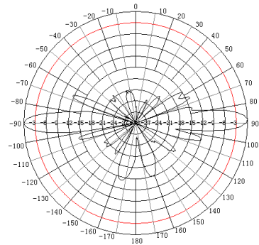
E Plane
