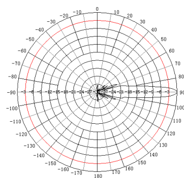
E Plane
