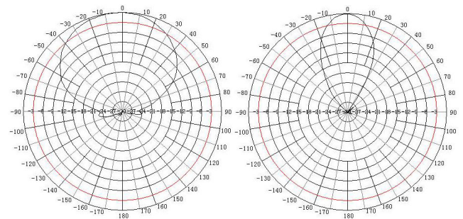
H Plane
