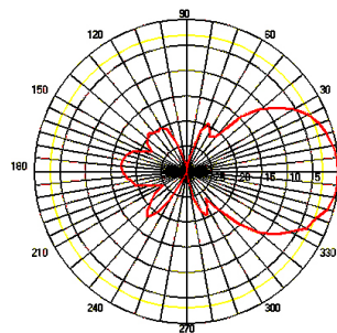
E-Plan@1800MHz
