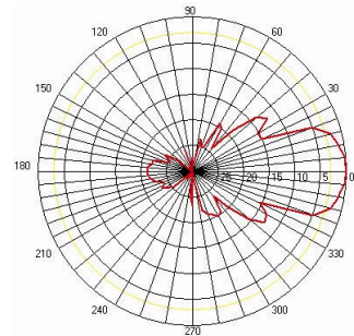
Typical Pattern@1200MHz
