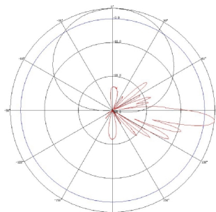
870~960MHz: ±45° Polarization
