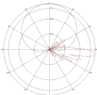
824~896MHz: ±45° Polarization
