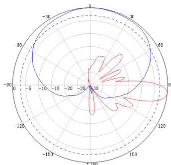
Pattern(Single Column) H Plane(Blue) E Plane(Red)
