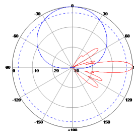
870~960MHz: ±45° Polarization
